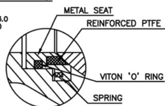
FIRE SAFE DETAILS-'B'
