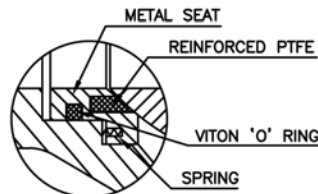
FIRE SAFE DETAILS-'B'
