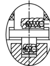
DETAILS-'A' ANTISTATIC DEVICE
