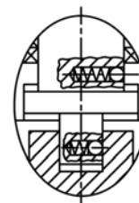
DETAILS-'A' ANTISTATIC DEVICE
